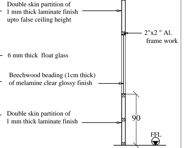
SECTIONAL ELEVATION A,A'
